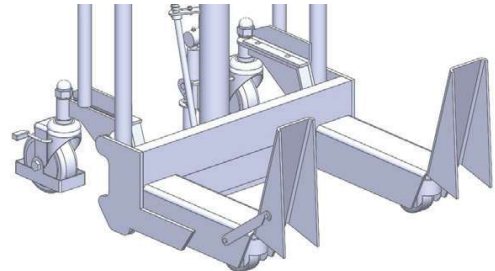
Flip Stops in the Transport Position
